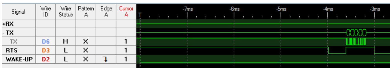
Figure 7: Wake-up from shutdown
